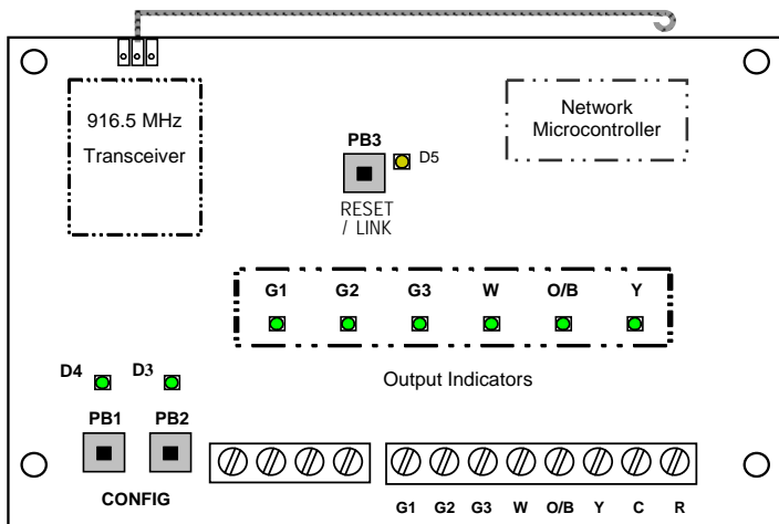
Figure 10 – Model 122 PTAC Wireless Control Node
