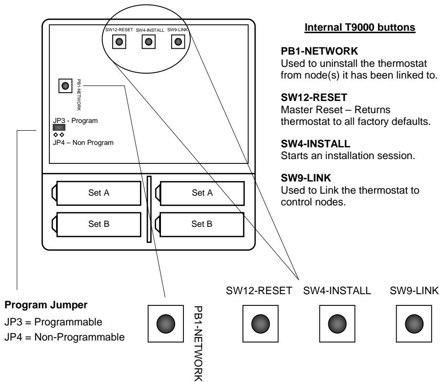
Figure 8 – Internal Buttons
