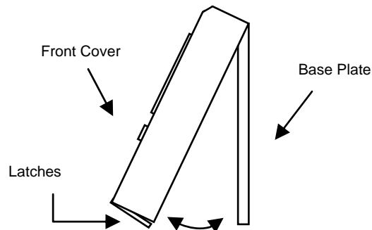
Figure 2 — Opening Thermostat
