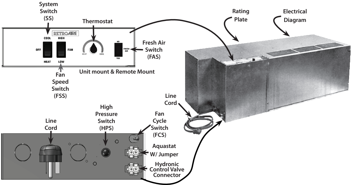
Figure 2 R80C | R80H chassis
