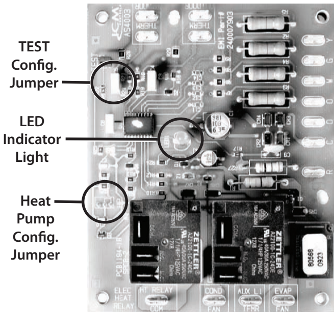
Figure 4 - Control Board
