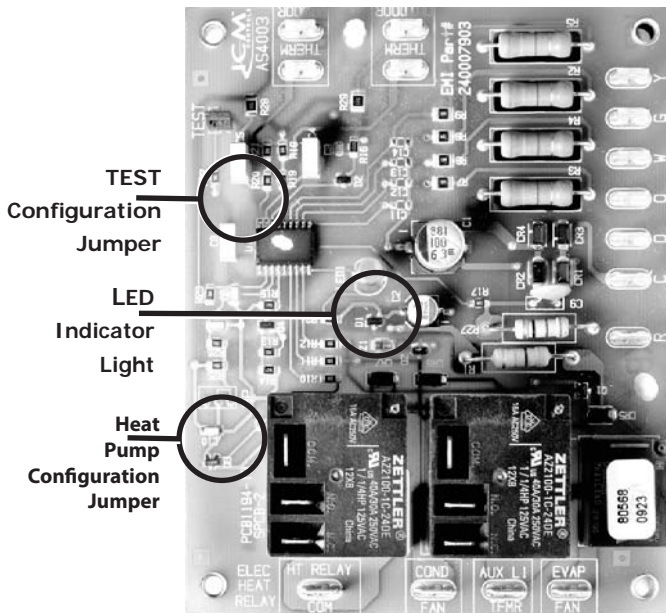
Figure 5 Control Board
