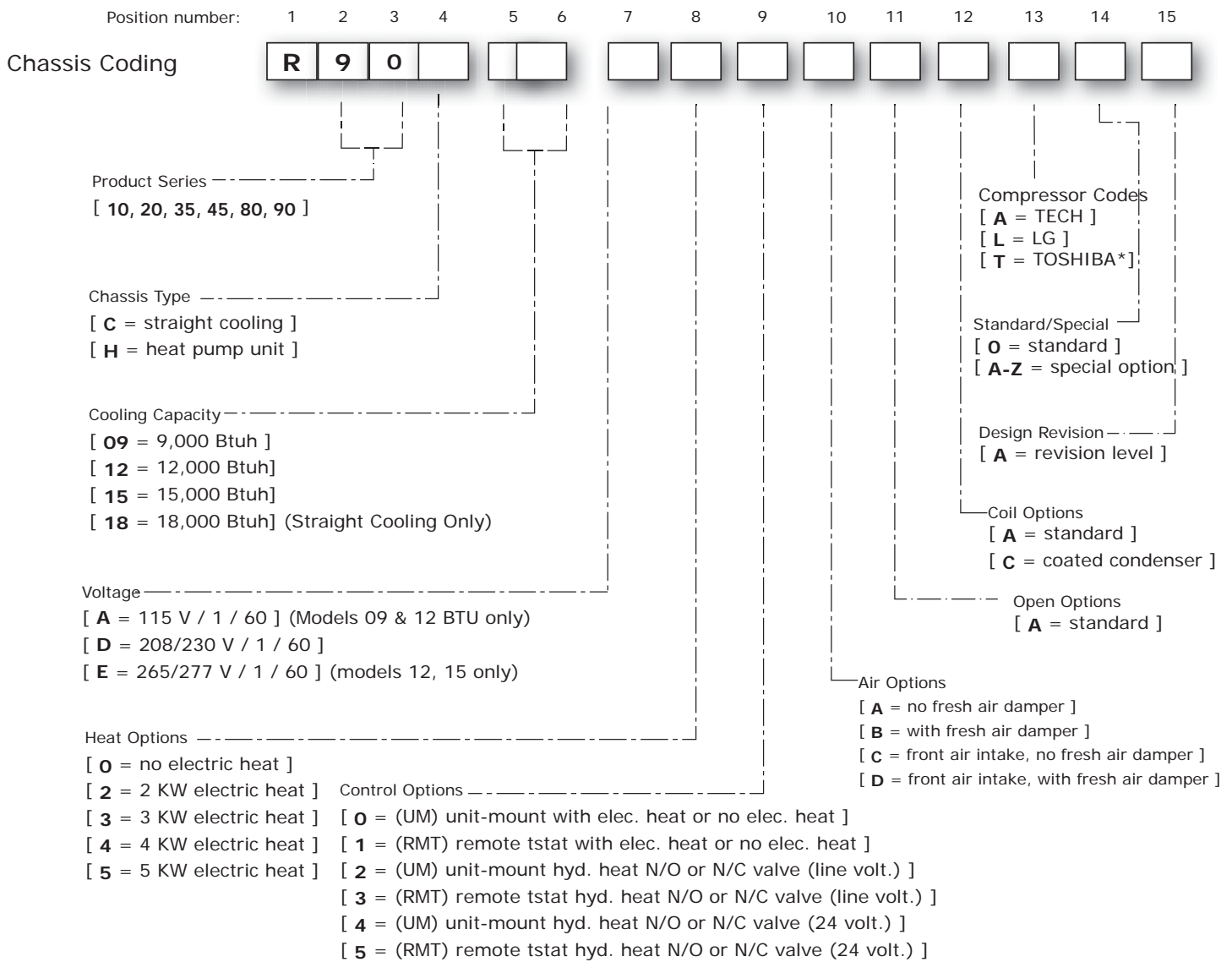
Figure 4 Model Coding
