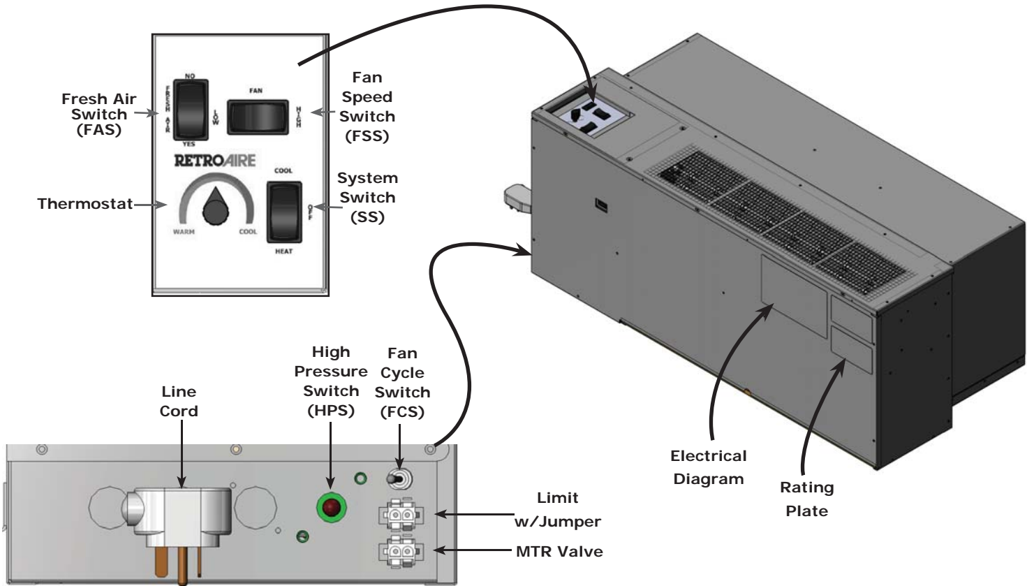
Figure 2 R24C | R24H Chassis
