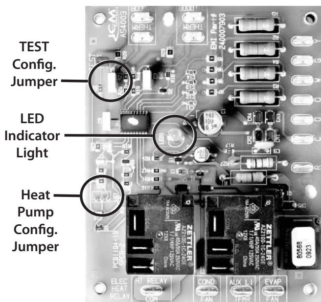
Figure 4 - Control Board
