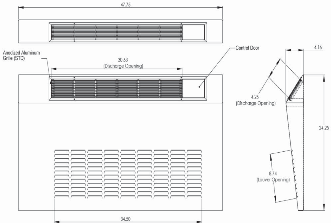
Figure 2 R15 Cabinet Front
