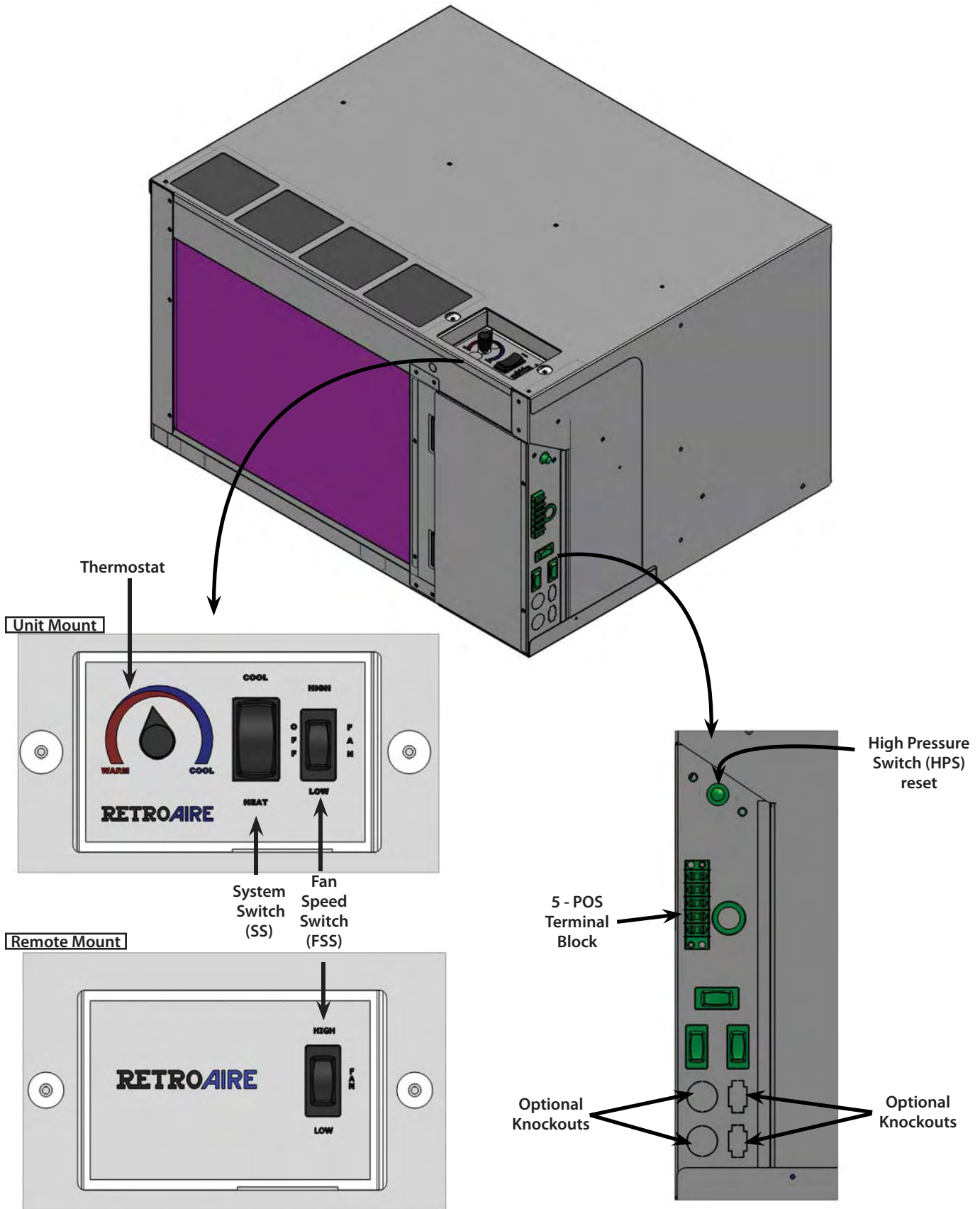
Figure 1 R40C chassis
