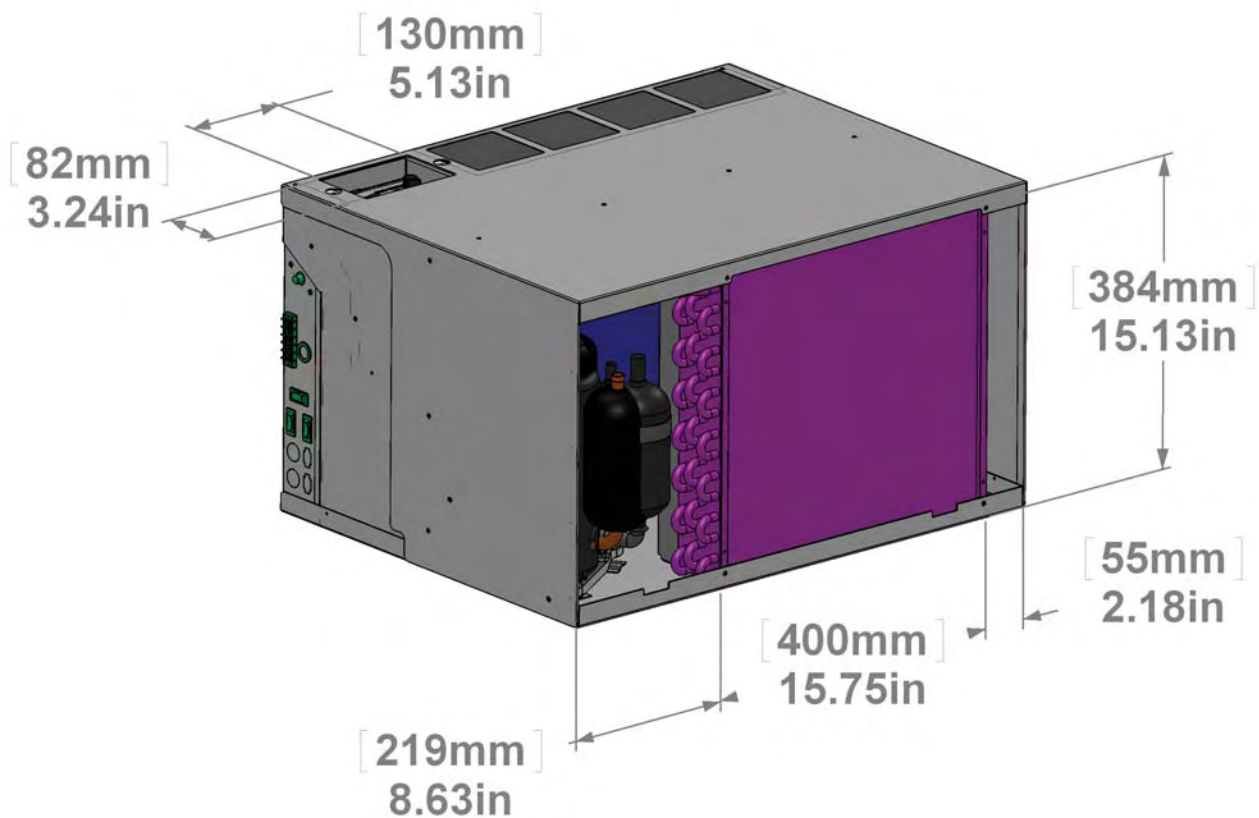
Figure 3 R40C Dimensioned Rear View
