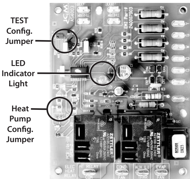
Figure 4 - Control Board
