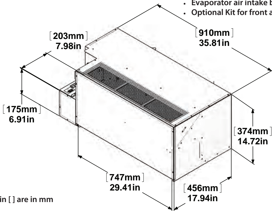
Figure 2 R90C | R90H chassis
