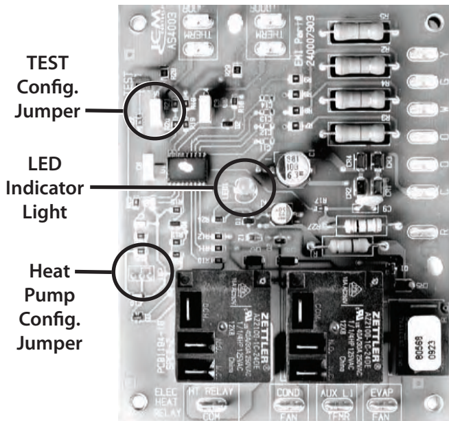
Figure 6 - Control Board
