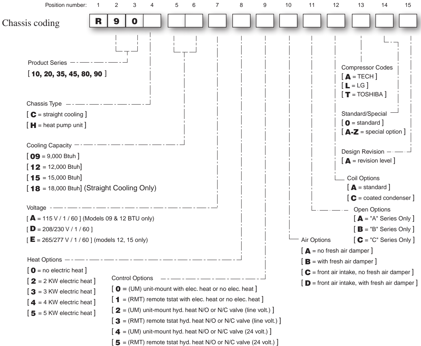
Figure 4 Model coding
