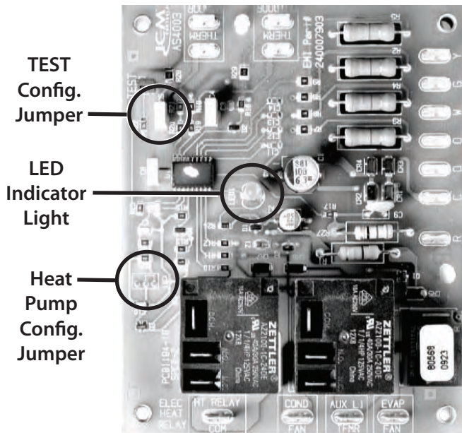
Figure 5 - Control Board
