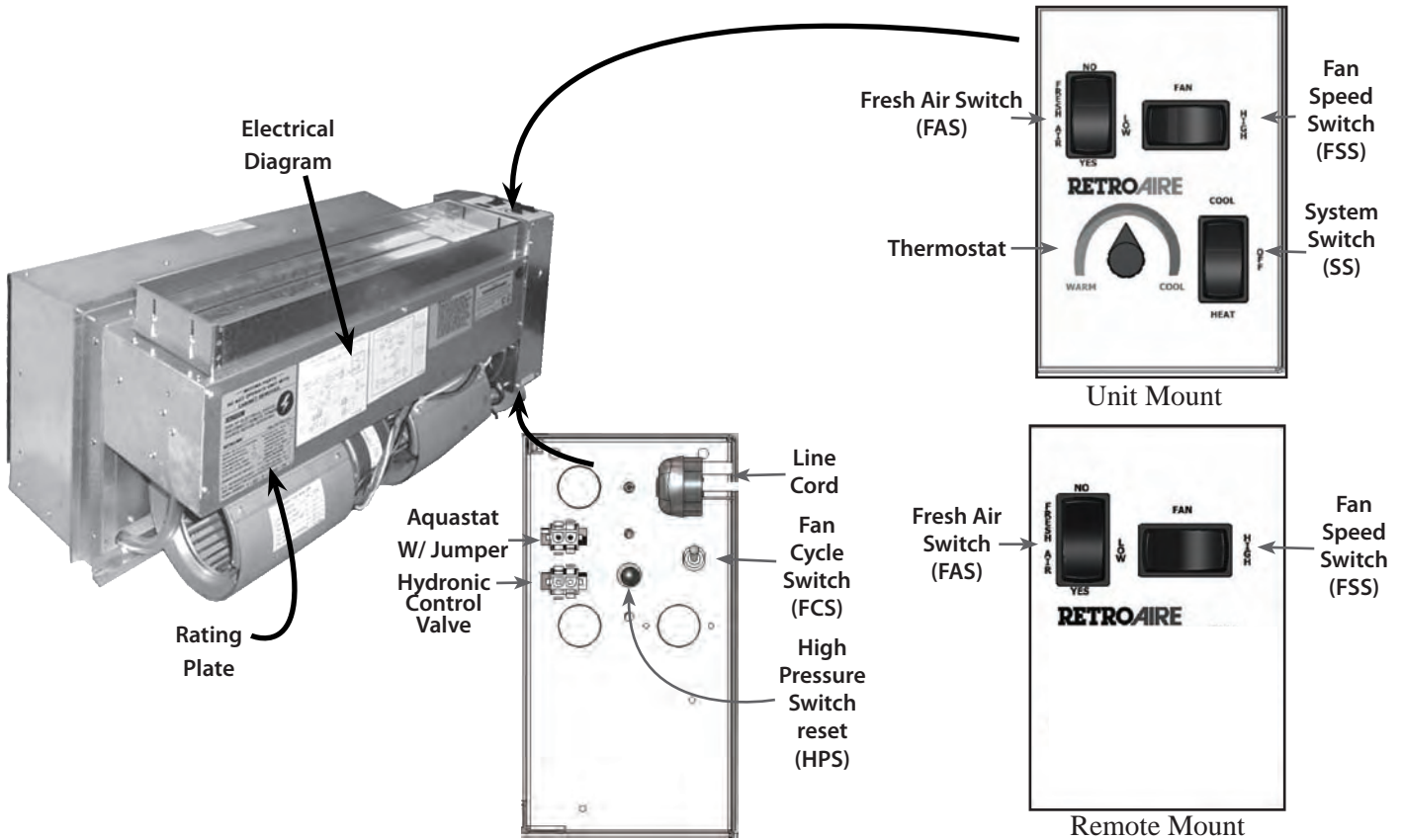
Figure 2 R45C | R45H chassis
