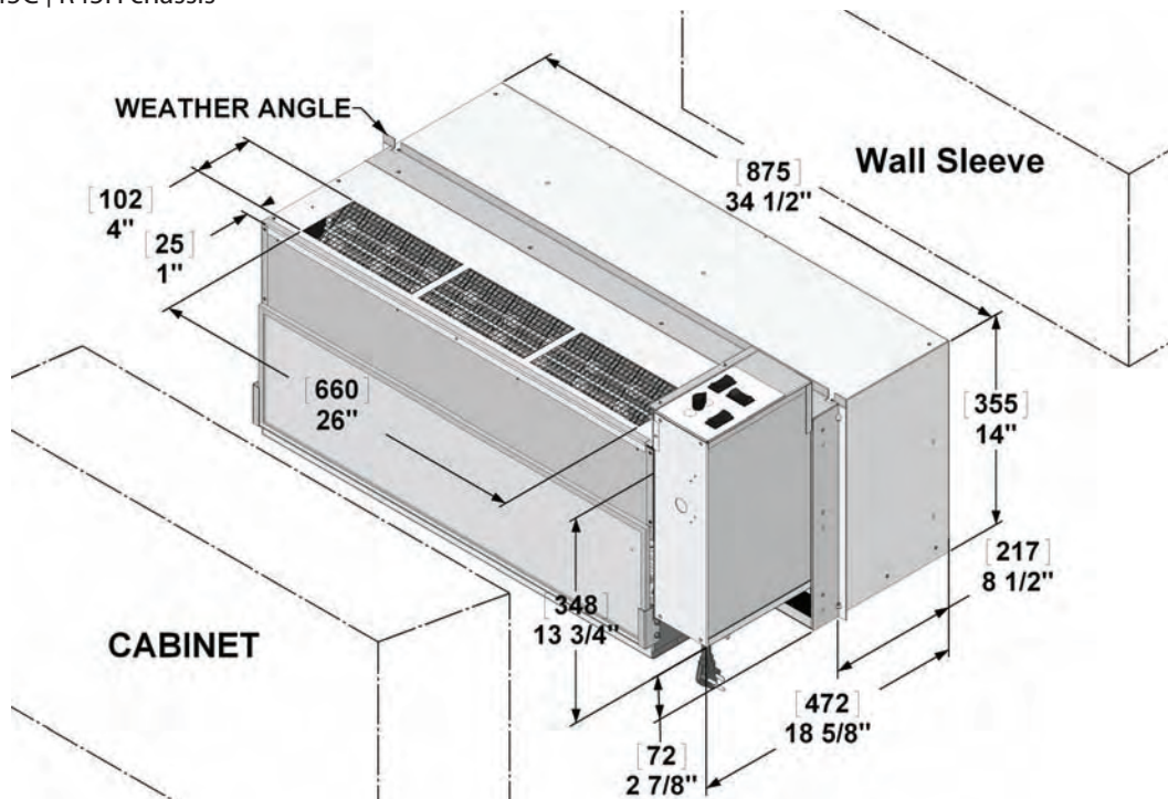
Figure 2 R45C | R45H chassis
