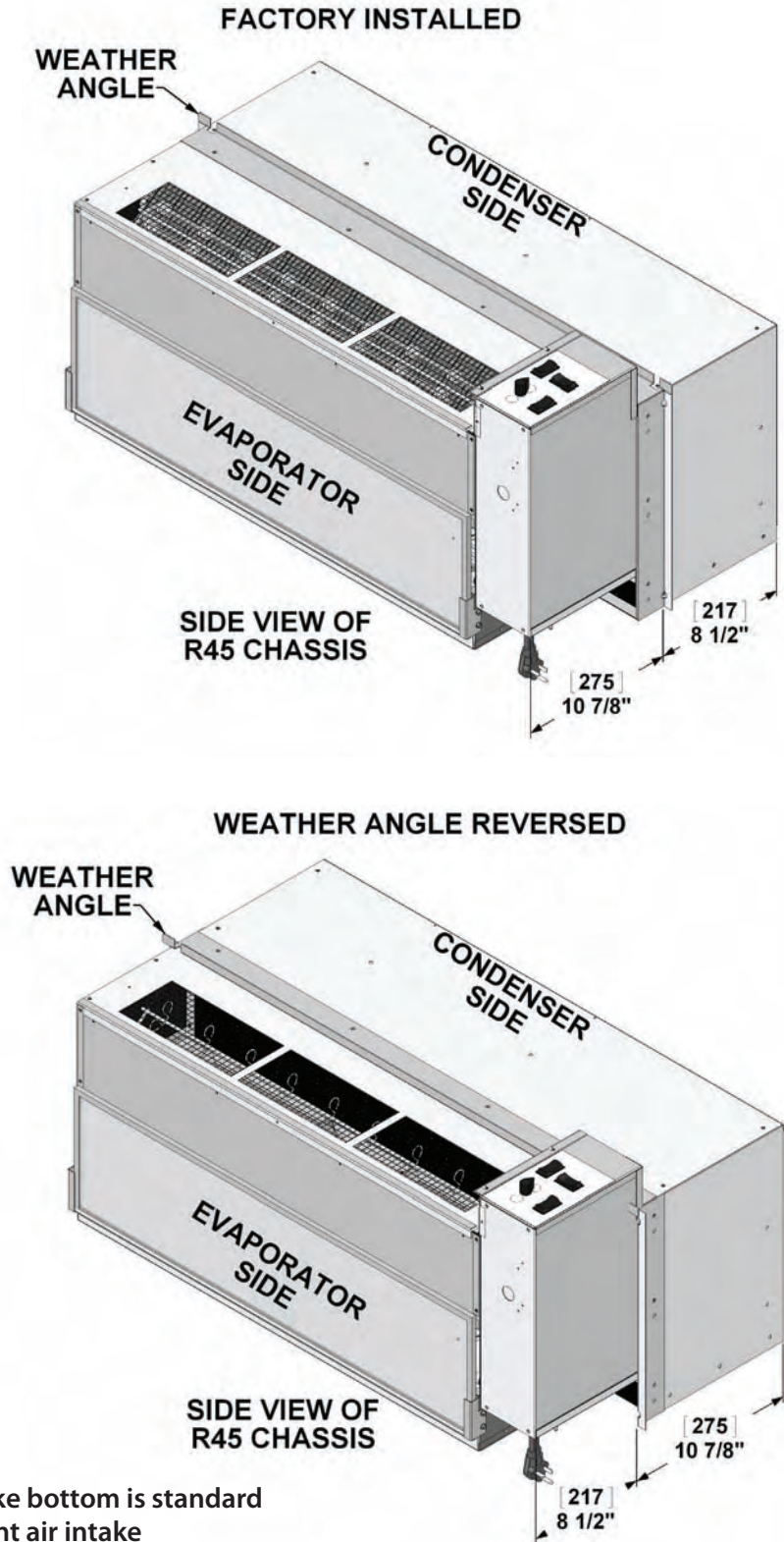
Figure 3 R45C | R45H Weather Angles
