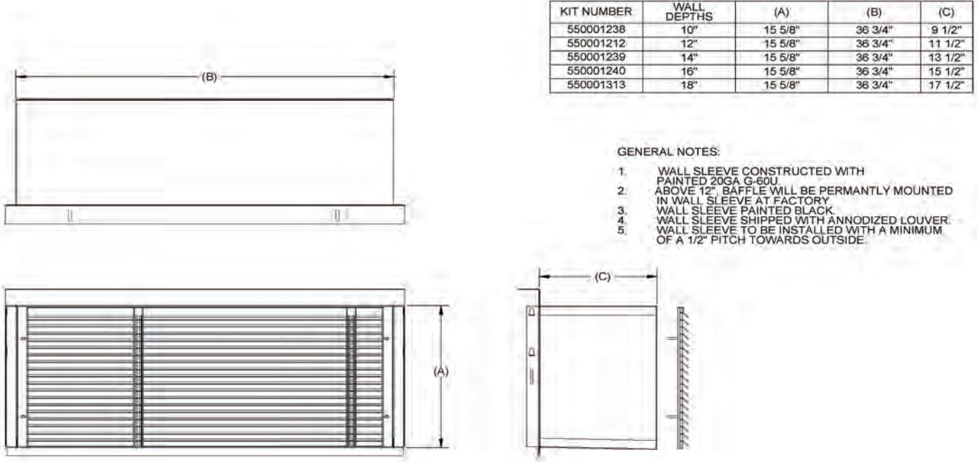
Figure 3 R22C | R22H Wall Sleeve
