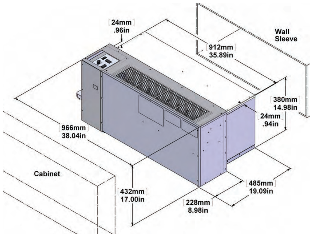
Figure 2 R22C | R22H chassis
