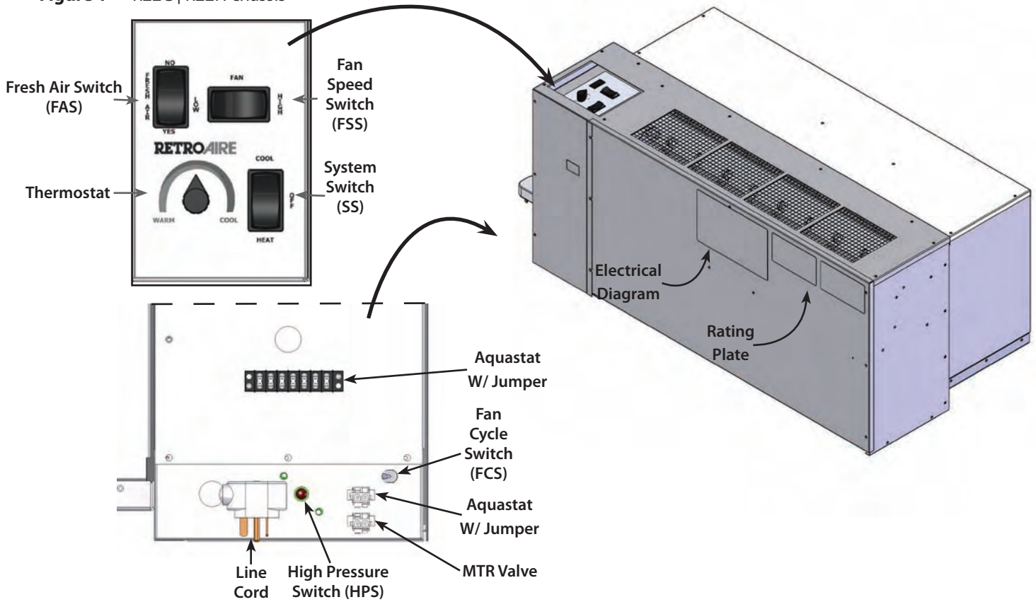
Figure 1 R22C | R22H chassis
