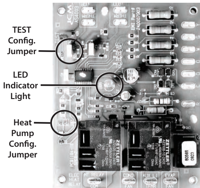
Figure 6 - Control Board
