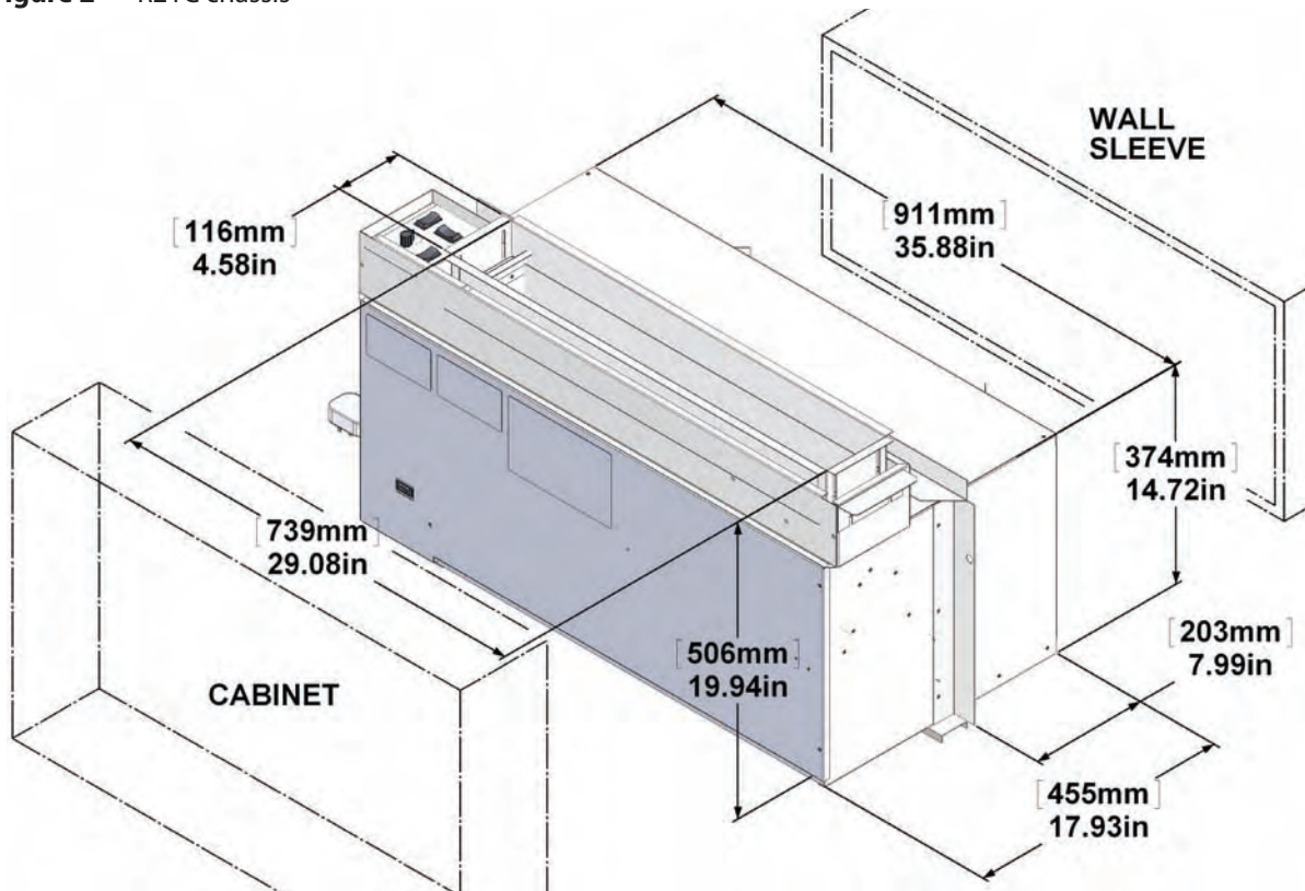
Figure 2 R21C chassis
