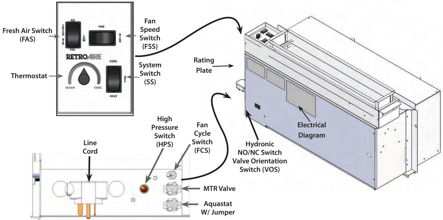
Figure 2 R21C chassis
