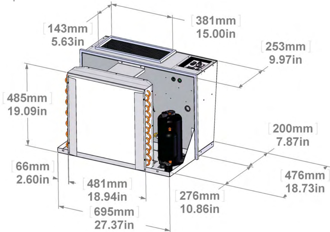
Figure 3 R25C | R25H chassis Dimensions Rear
