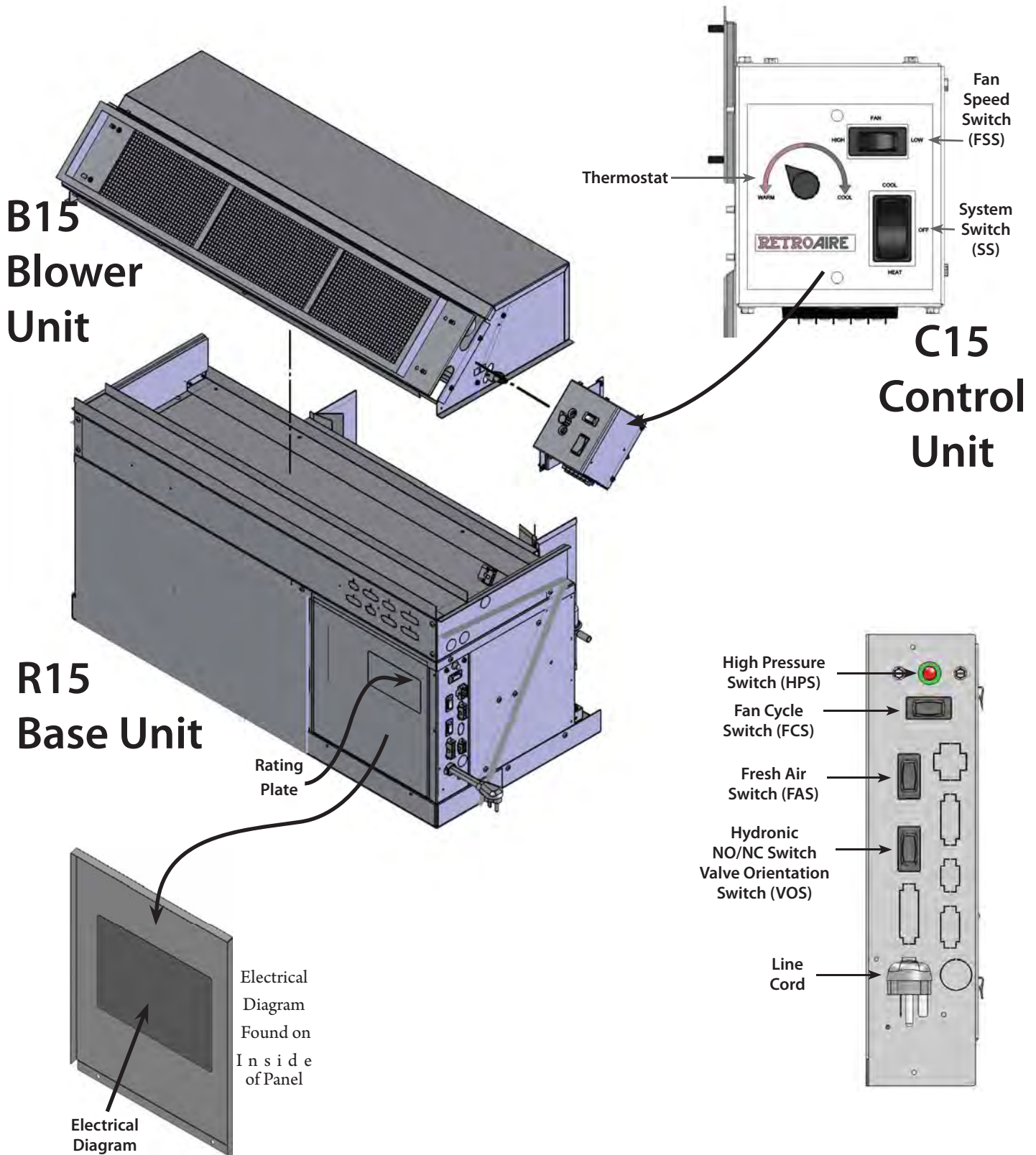
Figure 1 R15C chassis
