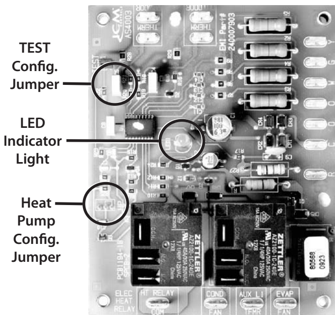
Figure 3 - Control Board
