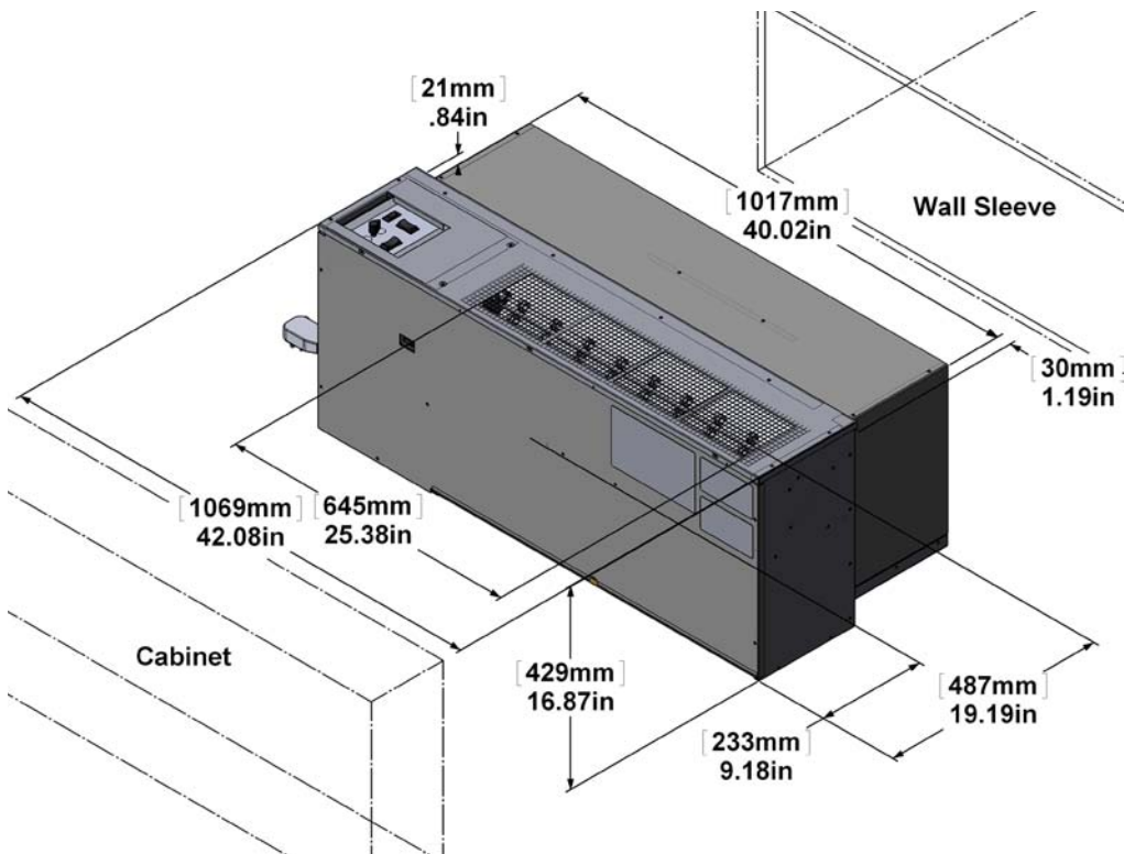
Figure 2 R24C | R24H chassis
