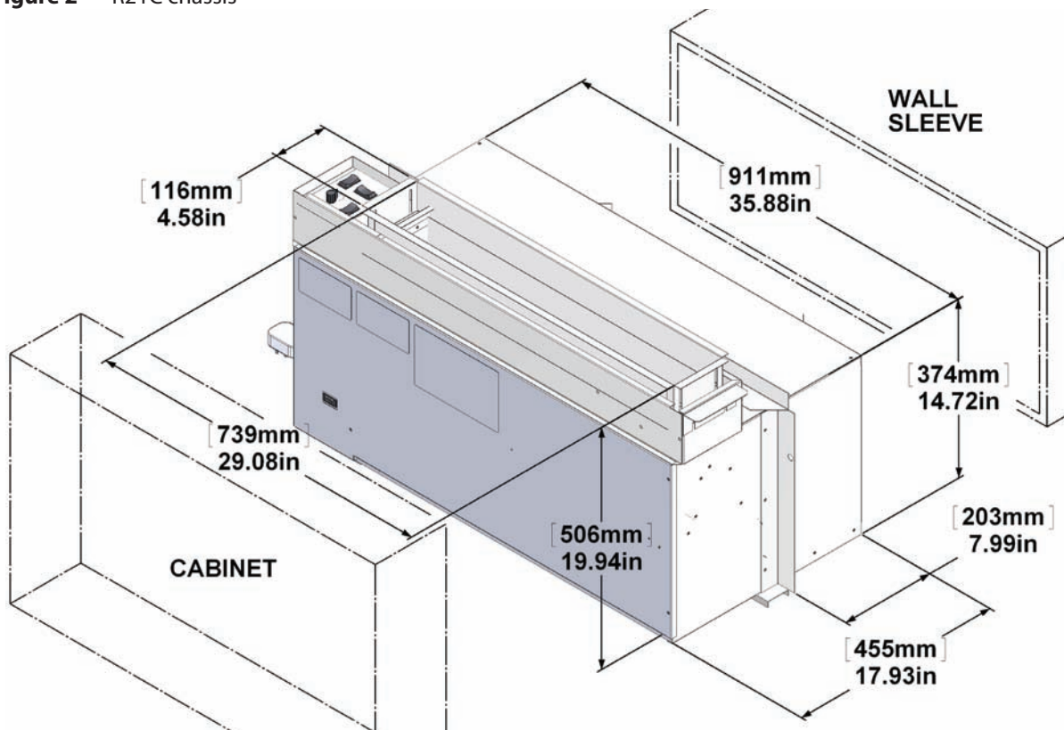
Figure 2 R21C chassis
